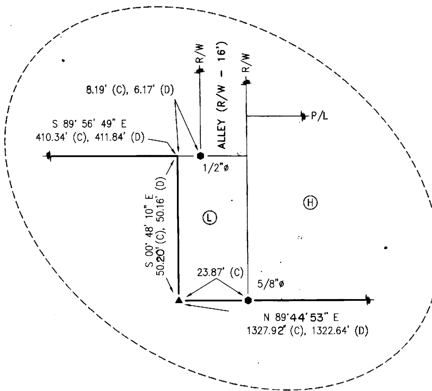
DETAIL SCALE - 1:20
