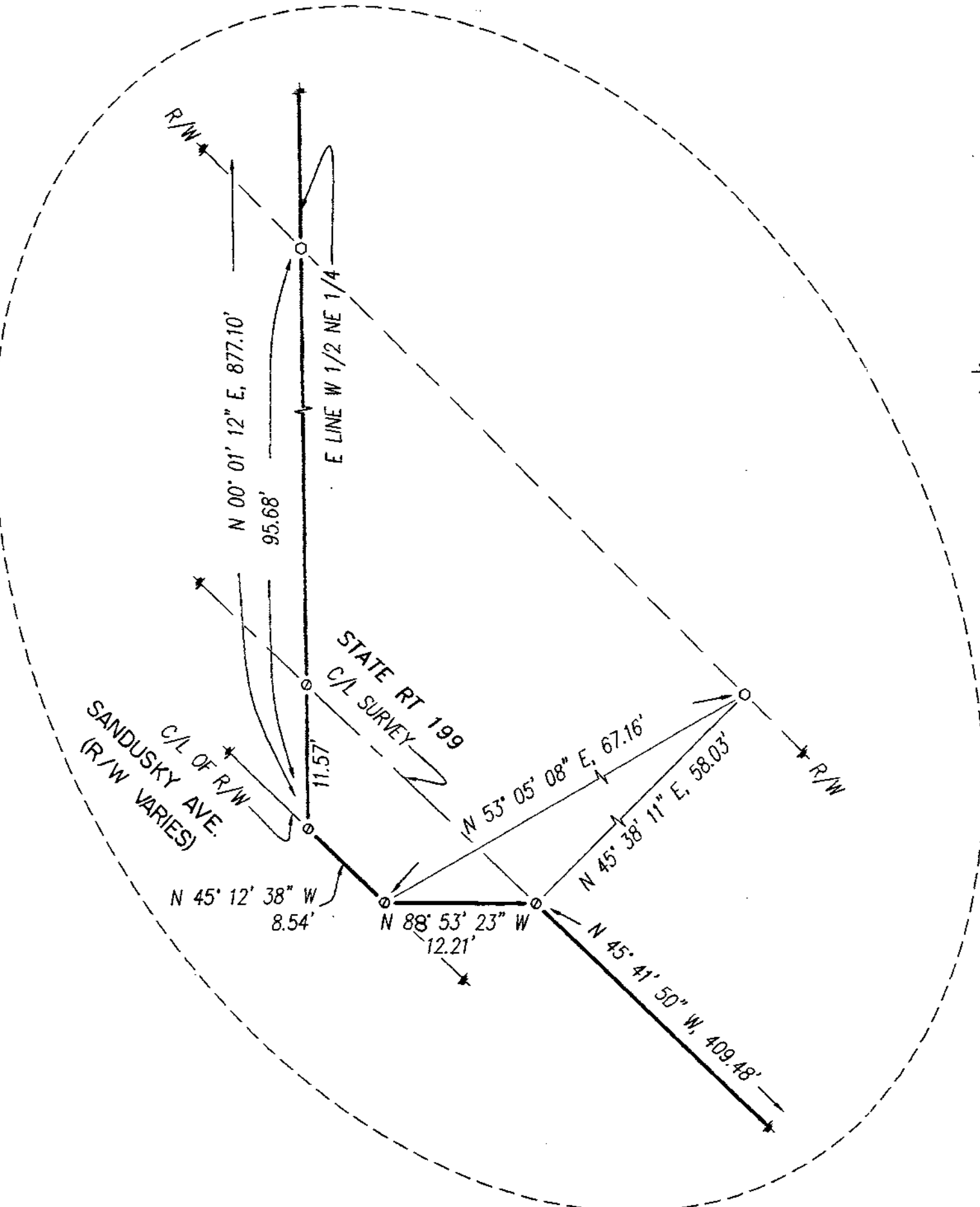
DETAIL 1" = 10'
