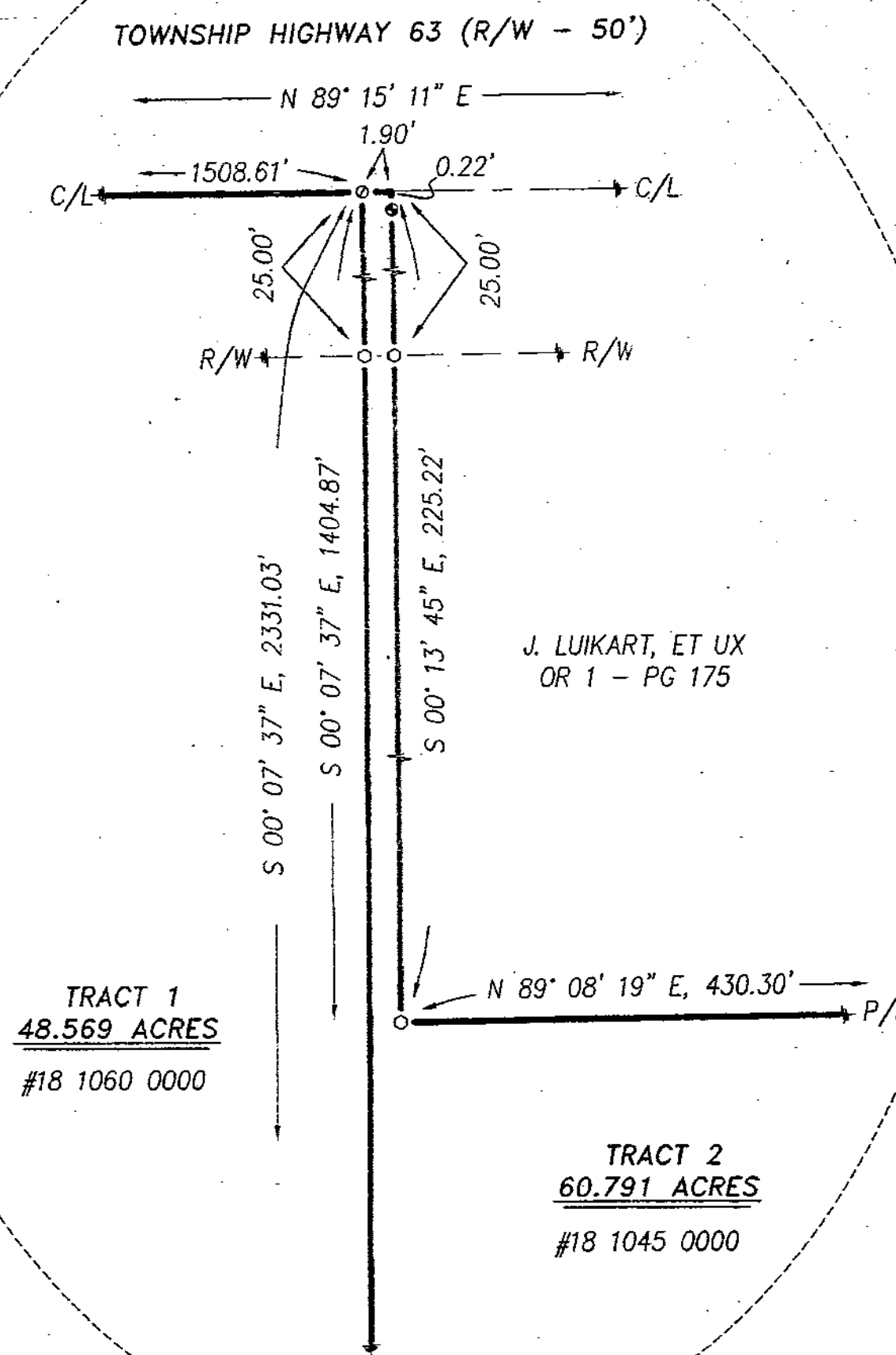
DETAIL 1" = 10'
